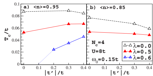
FIG. 4. (Color online) t' -dependence of T_c at (a) 5% and (b) 15% dopings for different values of the dimensionless EP coupling, \lambda [Eq. (2)]. A finite t' increases T_c in the under-doped region when EP coupling is present. For \lambda=0.6 in (a), the t'=0 point has been extrapolated from the data at temperatures larger than T_c .
